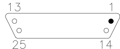
J1 PIN LOCATIONS
